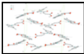
Fig. 2. Part of crystal structure of the title compound with N—H...O hydrogen bonds represented by dashed lines. Symmetry code (i): x, y - 1, z . H atoms not involved in intermolecular hydrogen bonding have been omitted.
